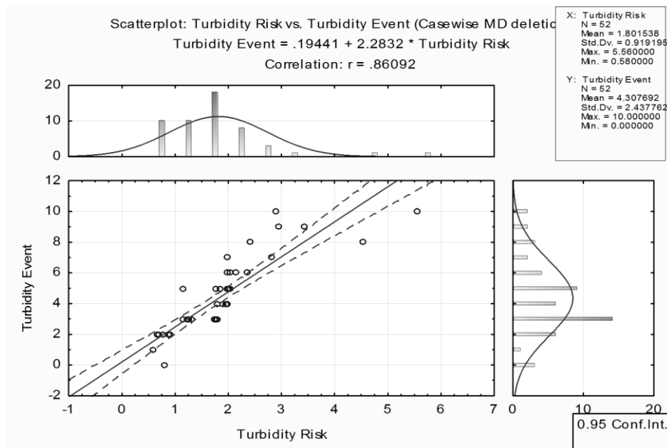
Figure 3. Statistical analysis of scatterplot data confirms a correlation between loads from sandy soil farms and turbidity events in the mill.
