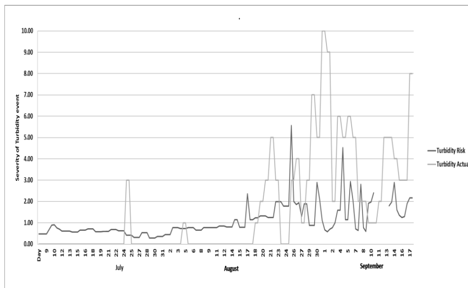
Figure 1. Covariance analysis of delivery frequency from ‘risk farms’ and actual subsequent turbidity events in the Malelane Mill from July to September 2013. The correlation coefficient obtained for this data was r^2=0.41 .
