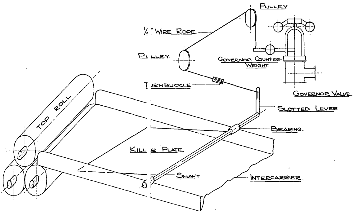
FIG. 2 MILL CONTROL
