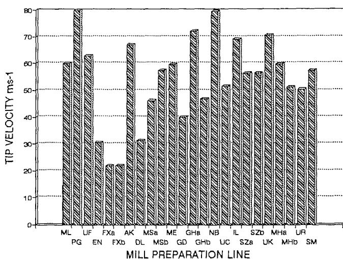
FIGURE 2 Distribution of the tip velocity of knives
