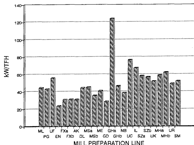
FIGURE 1 Distribution of specific power consumption of knives
