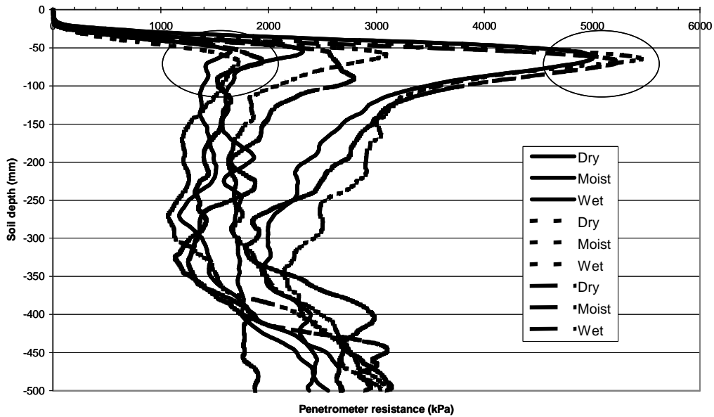
Figure 3. Penetrometer resistance for various depths and treatments as affected by soil water content. See peaks in the -50 to -100 mm soil depth layer. The highest three peaks are from dry soils and the lowest three from wet soils.
