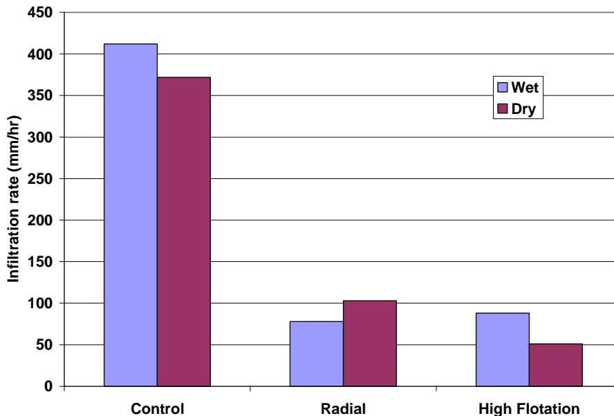
Figure 4. Water infiltration rates measured in the interrow area for three treatments and two water regimes.
