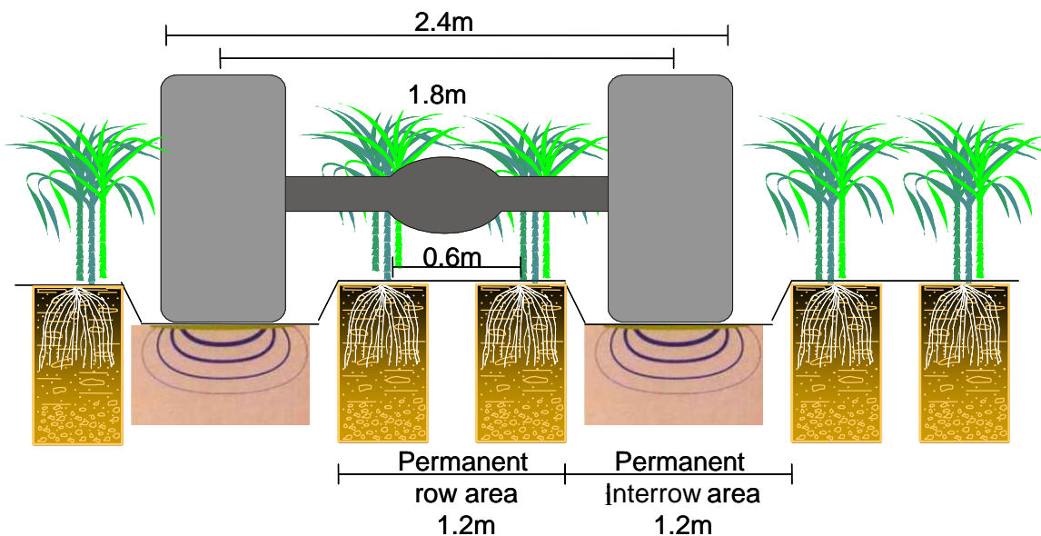
Figure 1. The 1.2 m interrow spacing combined with a 0.6 m row spacing arrangement that should be suitable for most farms.
